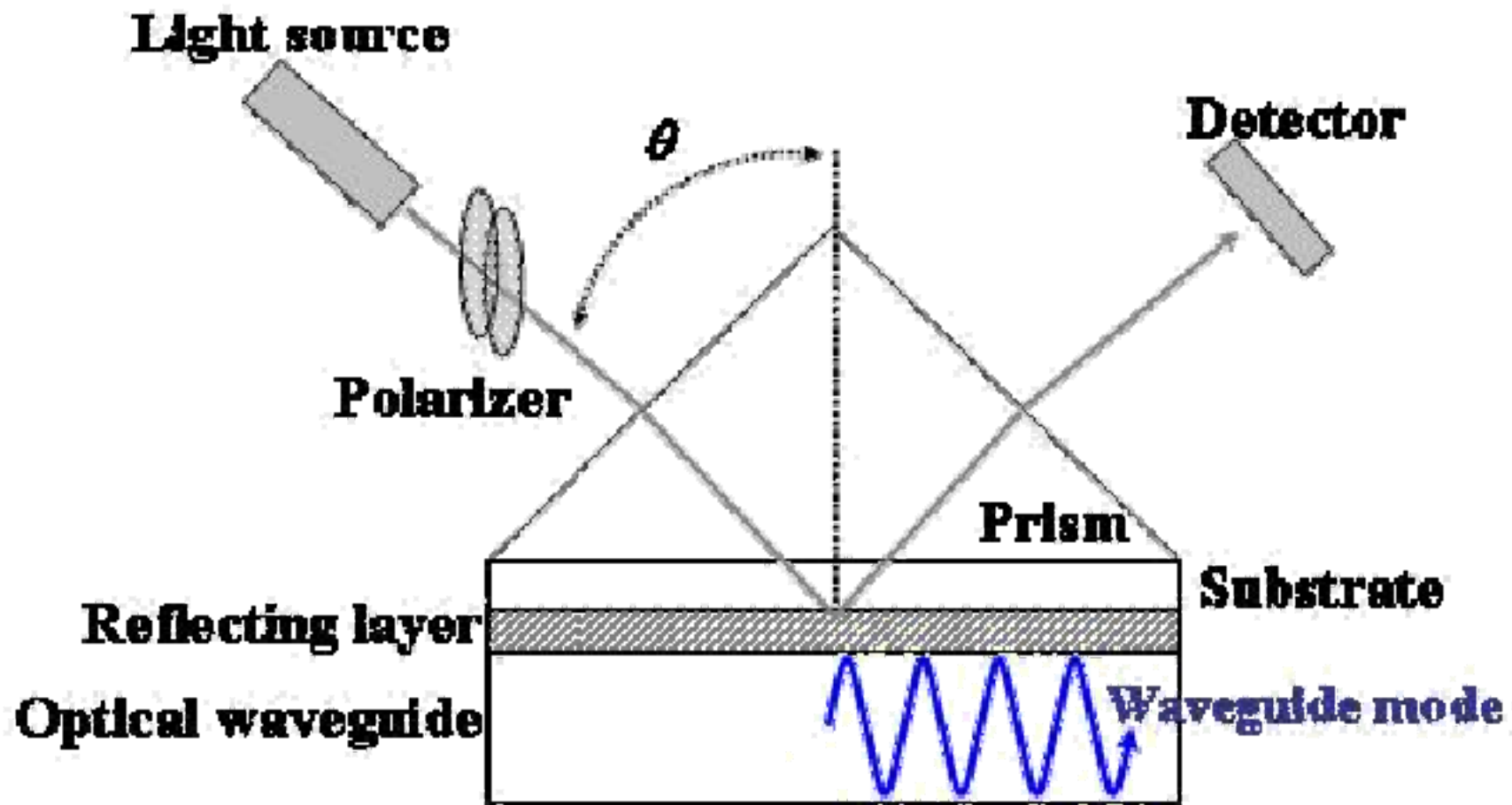
A waveguide-mode sensor
