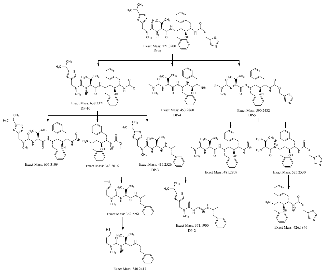
Fig. S2 Fragmentation pathway of DP-2, DP-3, DP-4, DP-5 and DP-10.
