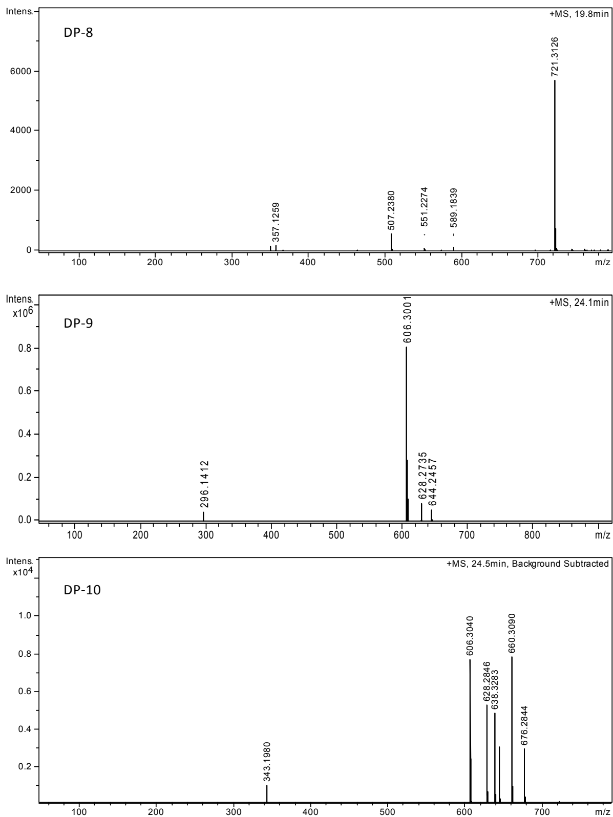
Fig. S1 Line spectra of degradation products (DP-2-10).
