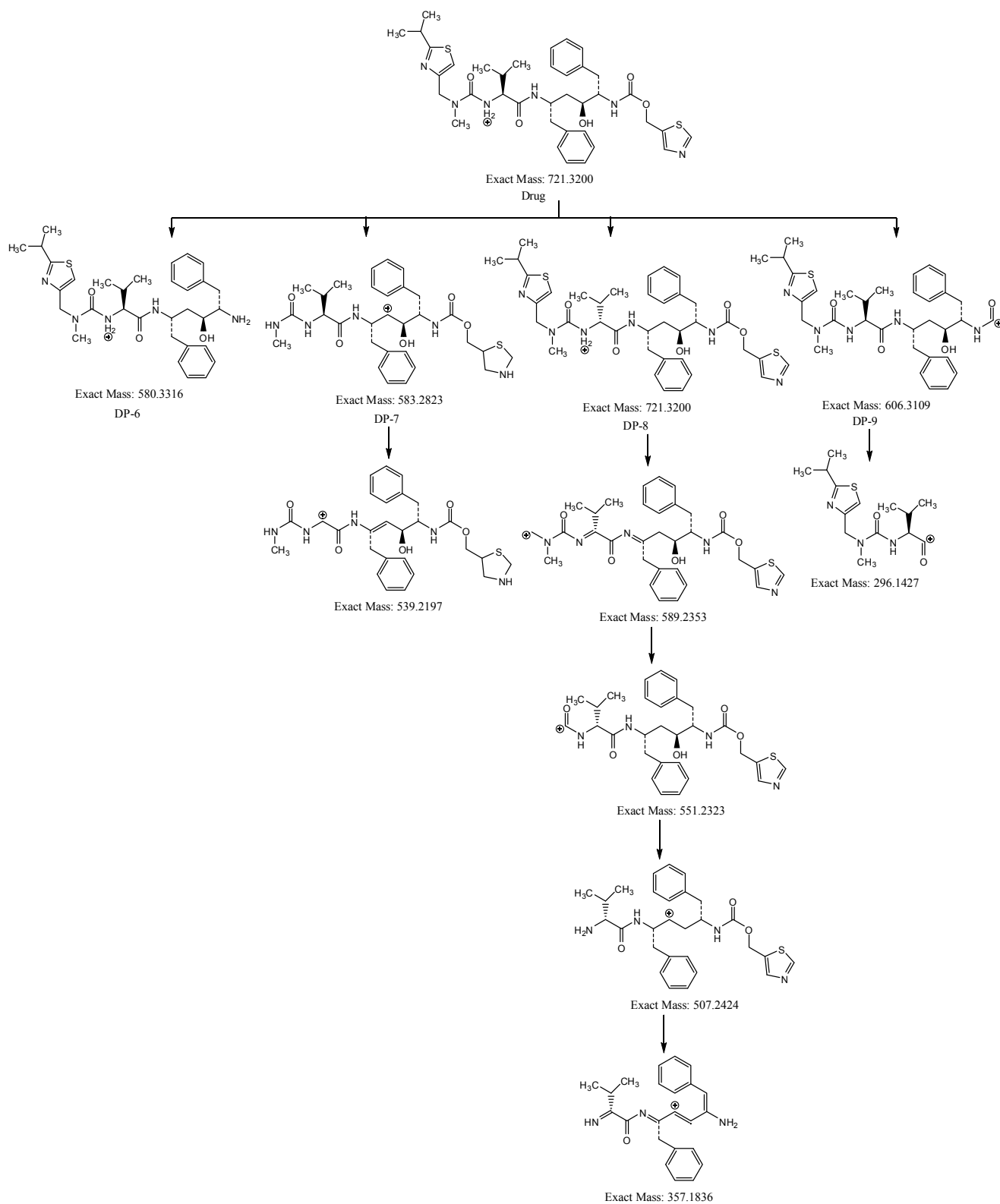
Fig. S3 Fragmentation pathway of DP-6, DP-7, DP-8 and DP-9.
