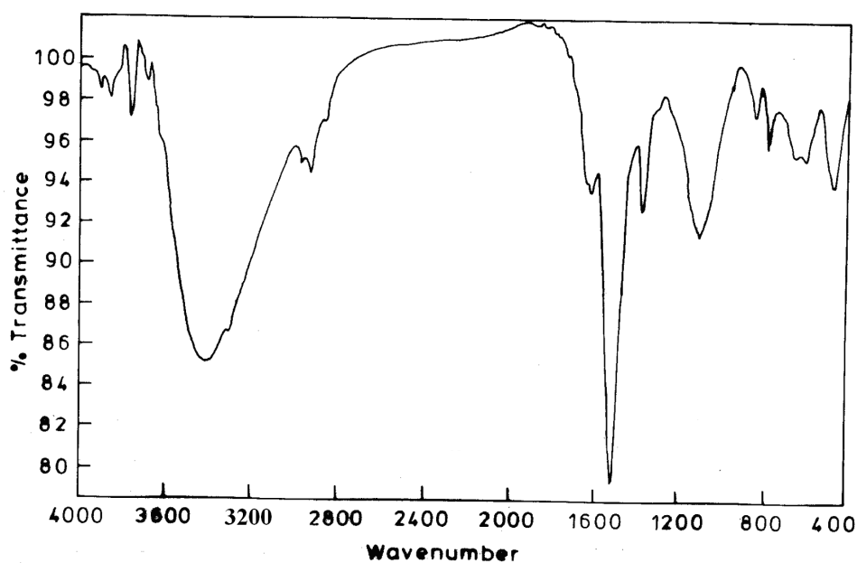
Set 4: Aniline polymerized with PAA over Nafion modified electrode in 1 M sulfuric acid (system 2).
