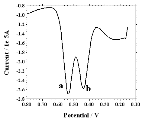
Fig.1 Square wave voltammograms of 5 \times 10^{-7} mol L -1 rutin (a) and 5 \times 10^{-6} mol L -1 quercetin (b) in NaAc-HAc (pH 4) at AuNPs/CNT/CPE. Other parameters are the same as Fig.7.
