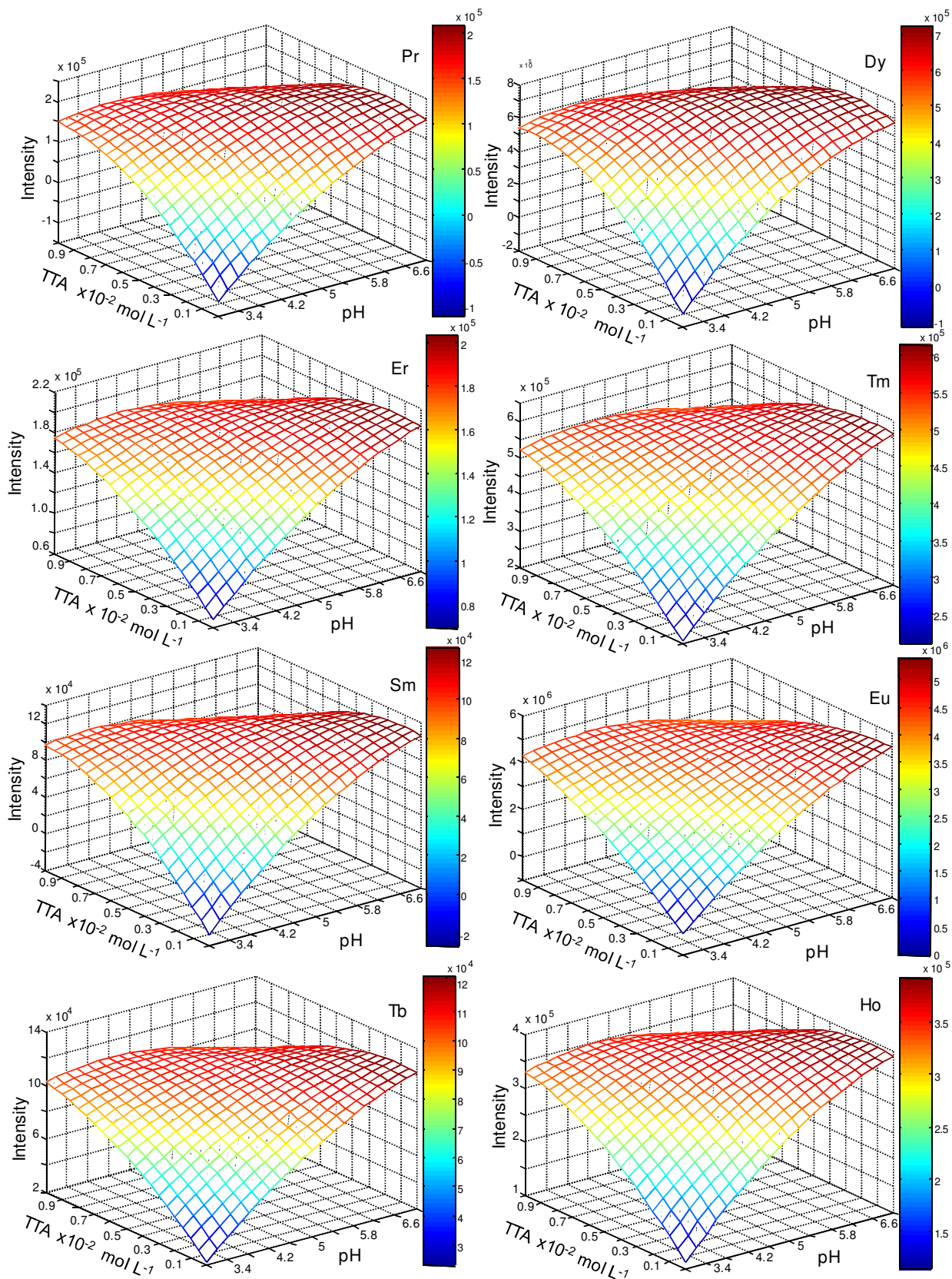
Fig. 2S Response surfaces of Pr, Dy, Er, Tm, Sm, Eu, Tb and Ho in solution submitted to CPE; 1-(2-thenoyl)-3,3,3-trifluoroacetone (TTA) is used as complexant.
