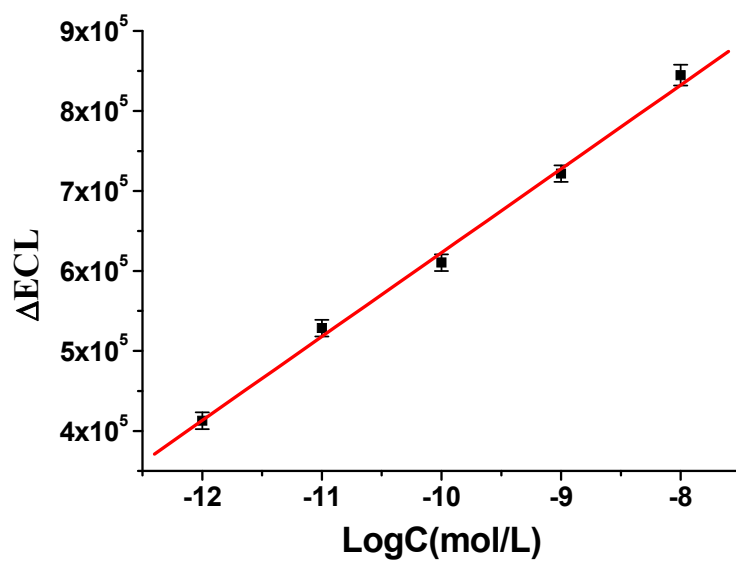
Fig. S3 Dependence of the ECL increasing versus the logarithmic concentration of LMG with 0.4 mM bimetallic ruthenium in 0.1 M borate buffer (pH 10) at Au electrode.
