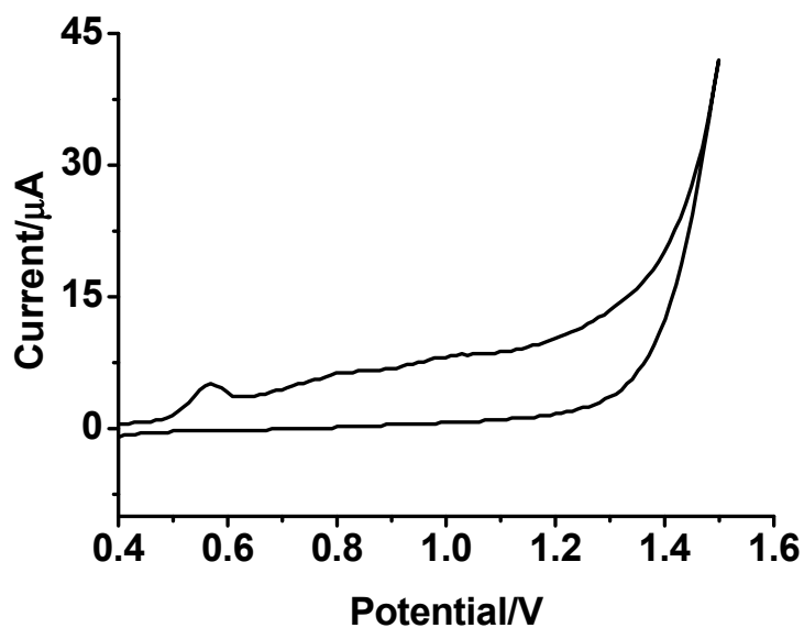
Fig. S1. Cyclic voltammetric curves of 1 mM MG in 0.1 M borate buffer (pH10) at Au electrode,
