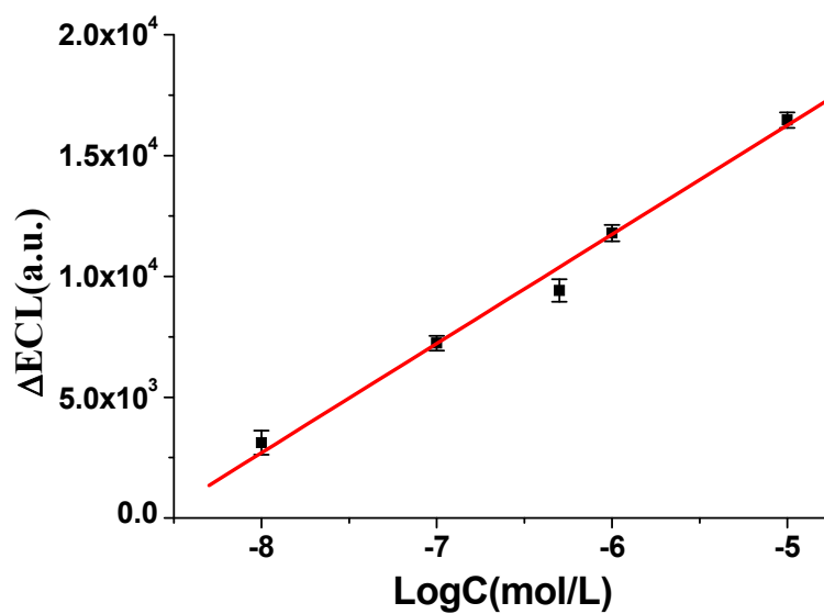
Fig. S2 Dependence of the ECL increasing versus the logarithmic concentration of LMG with 1 mM Ru(bpy) 3 2+ in 0.1 M borate buffer (pH 10) at Au electrode.
