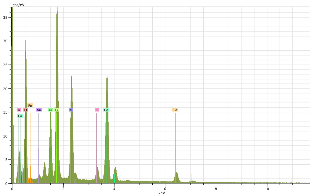
Figure ESI-4C: EDX spectrum obtained from Sample AT54A1-08
