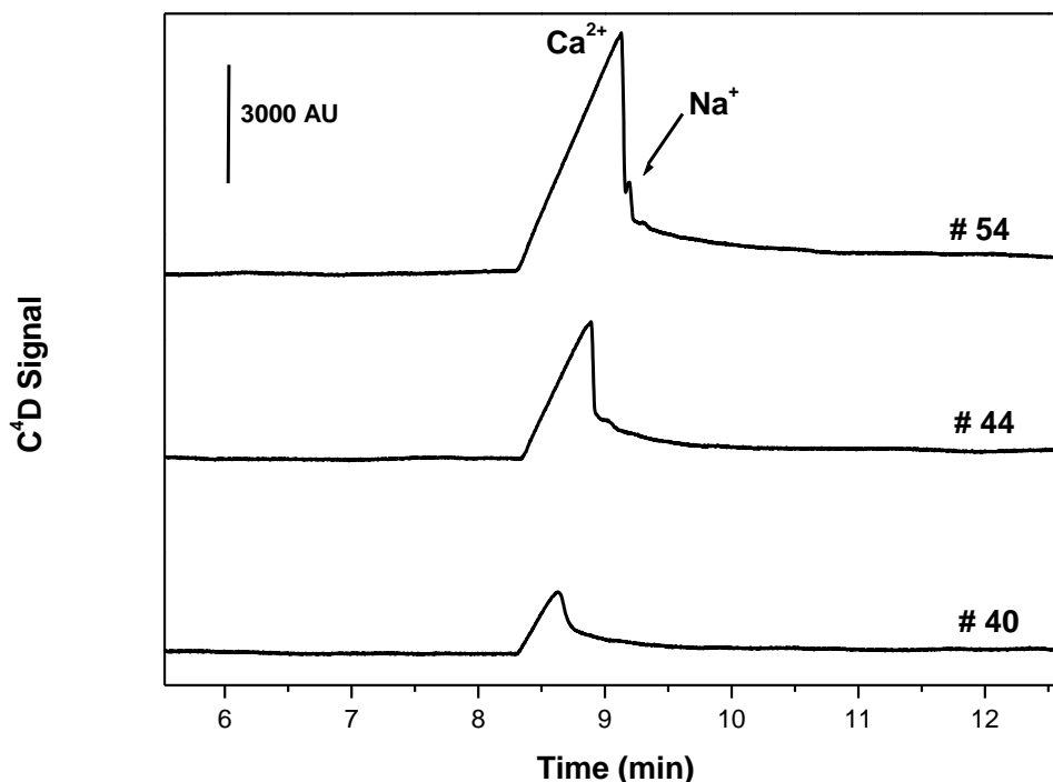
Figure ESI-2: Electropherograms of the Atacama's soil samples.
