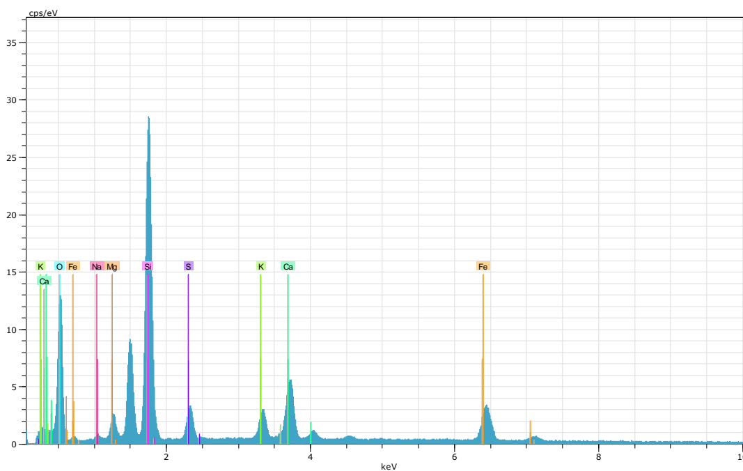
Figure ESI-4B: EDX spectrum obtained from Sample AT44B1-08
