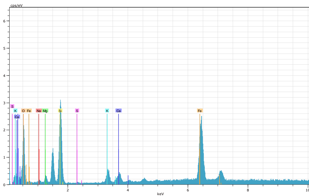
Figure ESI-4A: EDX spectrum obtained from Sample AT40B1-08
