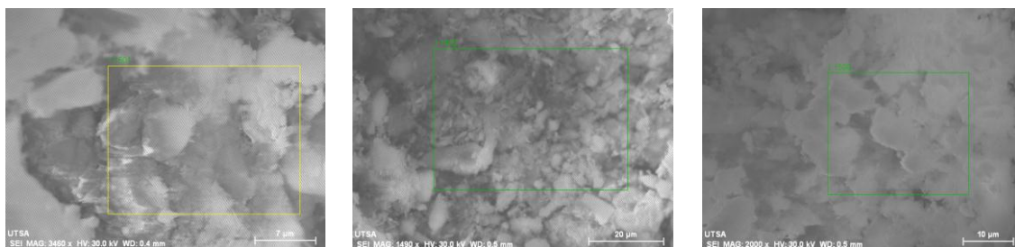
Figure ESI-3: Representative SEM images (30.0kV) of the soil samples obtained for the elemental analysis by EDX.
