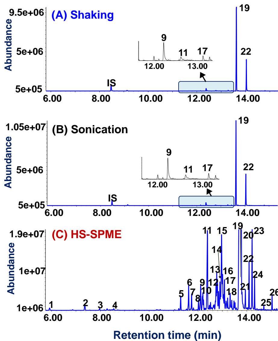
Supplementary Fig. 2. (A-C) TICs of volatiles and (D) extraction yields according to extraction methods
