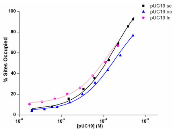
Figure S1- Percentage of sites occupied for L-arginine/plasmid pUC19 isoforms.
