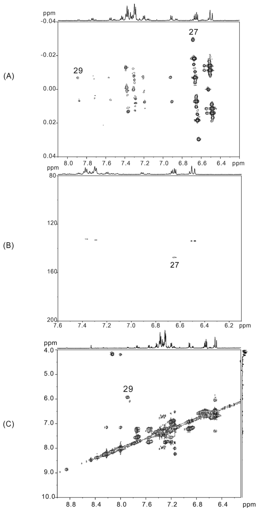
Fig. S1 2D NMR spectra for uridine and N-trans -feruloyltyramine
