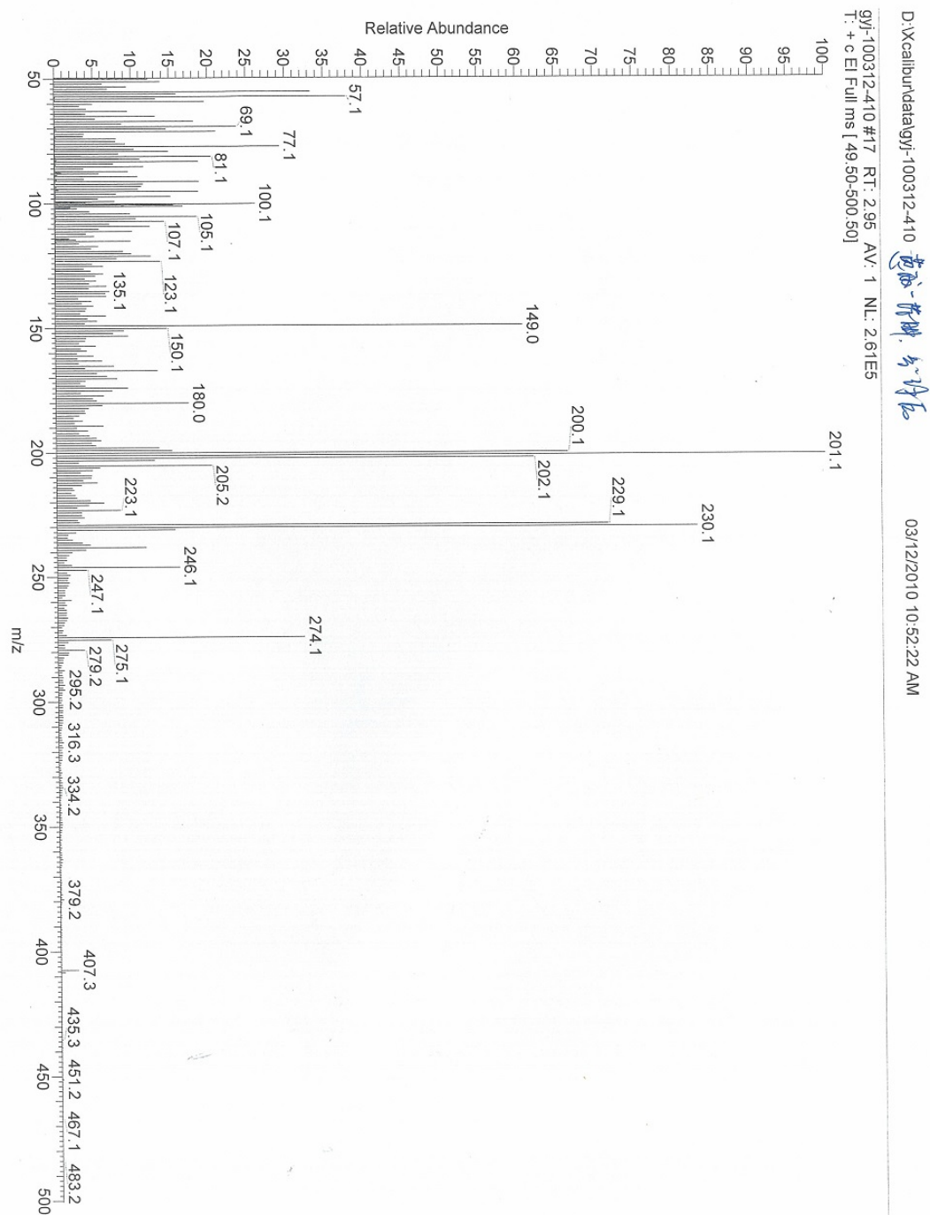
Mass spectrum of the final product of DPH with \text{OCl}^-
