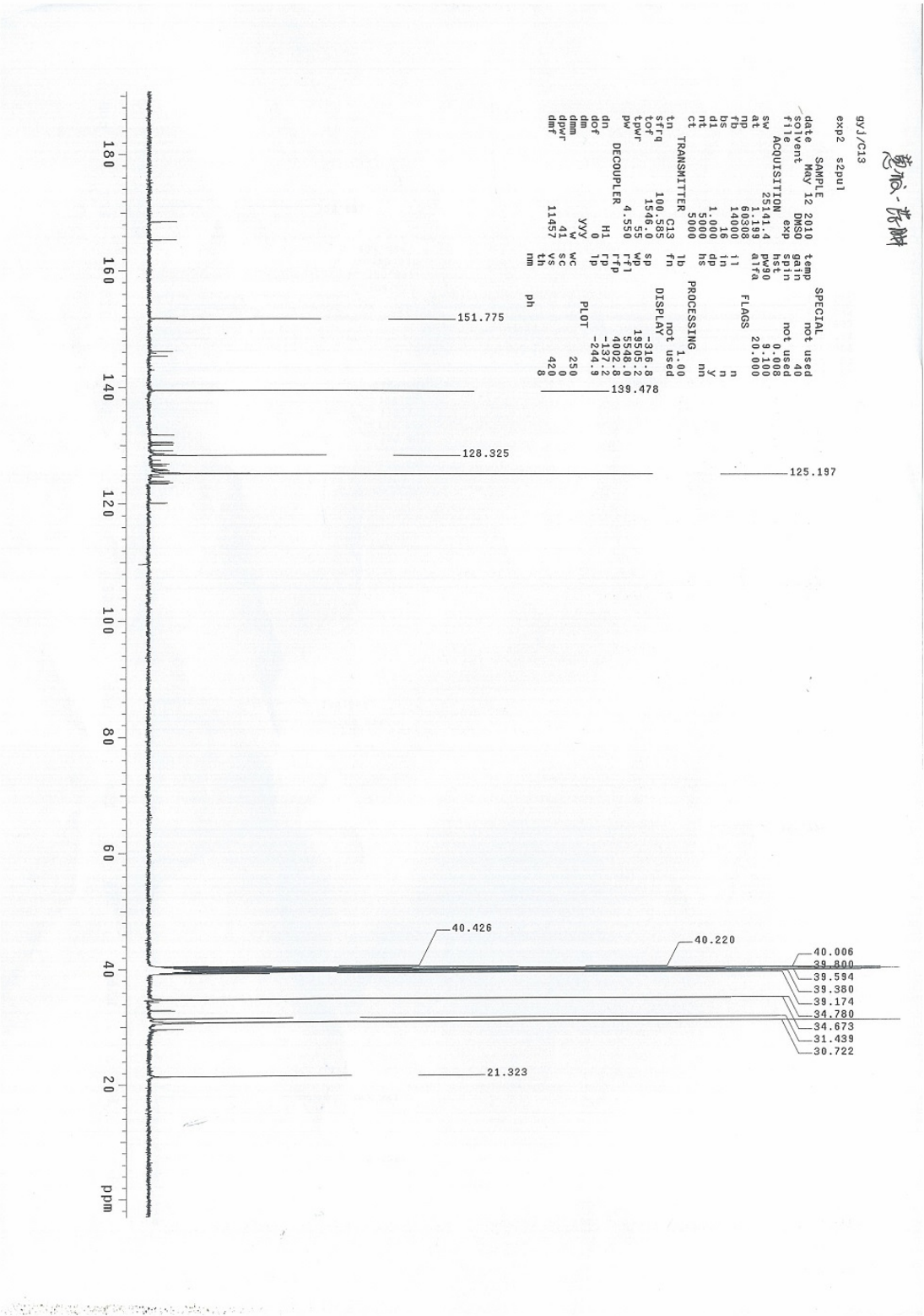
13 C-NMR spectrum of DPH
