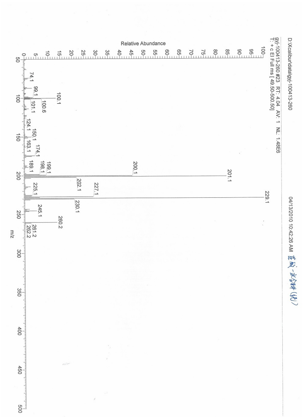
Mass spectrum of PZ
