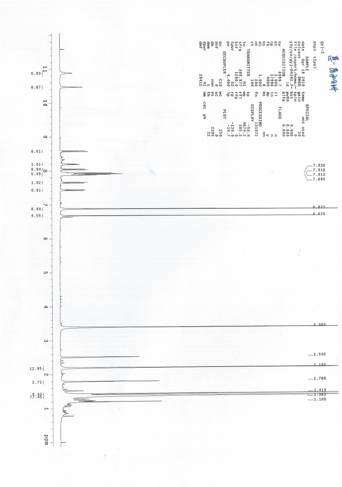
1 H-NMR spectrum of DPH
