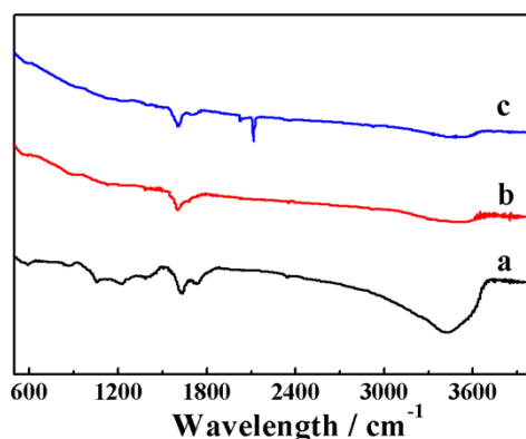
Fig. S2 FT-IR spectra of GO (a), GNs (b) and GdHCF/GNs (c).
