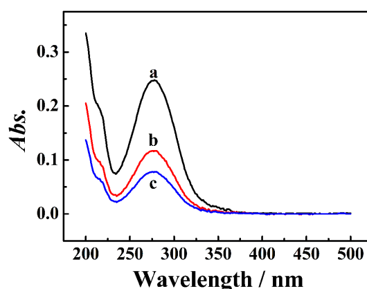
Fig. S4 UV-vis spectra of MP solution before (a) and after adsorption on GNs/GCE (b) and GdHCF/GNs/GCE (c), accumulation time: 5 min.
