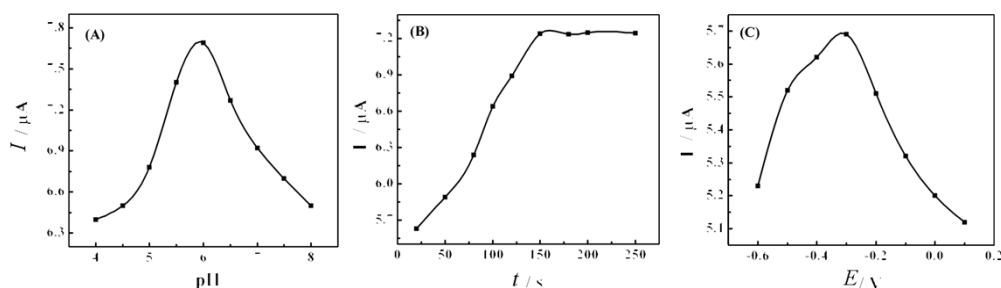
Fig. S5 Influence of pH value (A), accumulation time (B) and accumulation potential (C) on the DPV response of the GdHCF/GNs/GCE to 8 \mu M MP in 0.1 M PBS.
