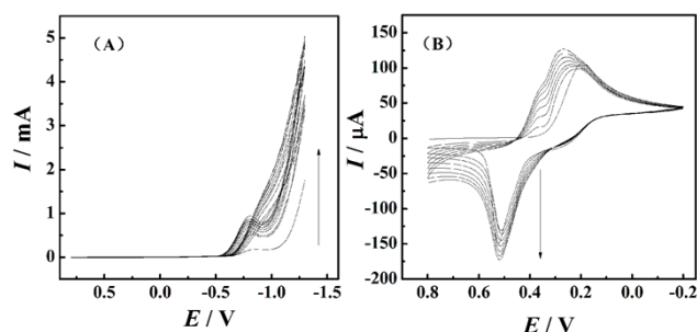
Fig. S1 The typical cyclic voltammograms of GNs (A) and GdHCF (B) deposition process on GCE.
