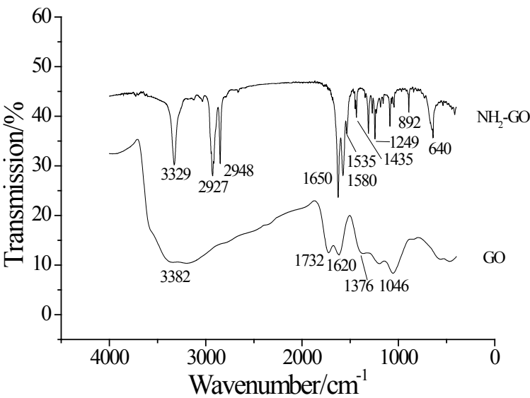
Fig. 1S FT-IR spectra of GO before (a) and after (b) amine modification
