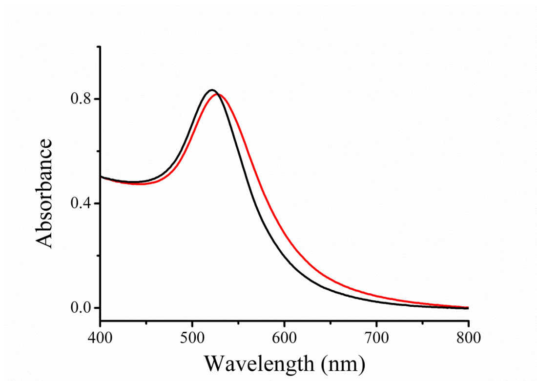
Fig. S1 UV-vis absorption spectra of BSA-absorbed gold nanoparticles before (black trace) and after (red trace) addition of 100 μM copper (II) ions.
