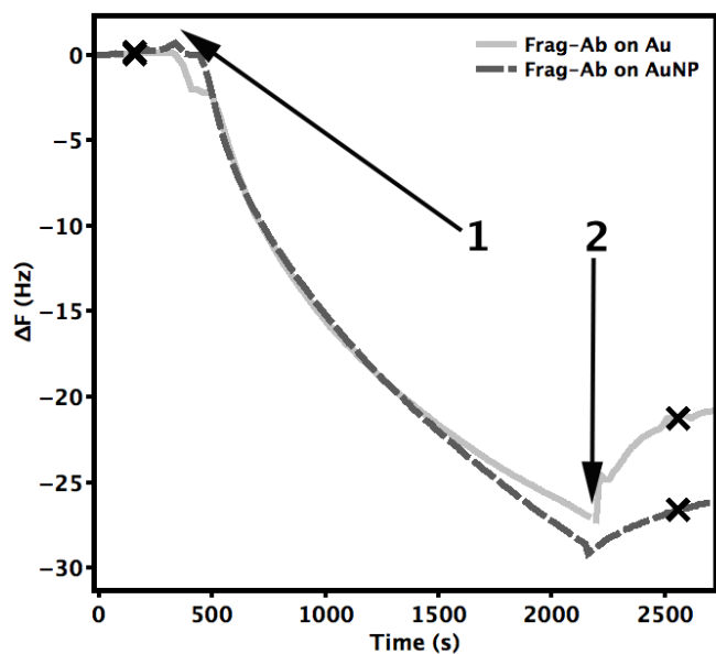
Figure S2. Frag-Ab/gp51 interaction on planar Au (grey line) and AuNP modified (black line) QCM-D sensor surfaces at 0.5 mg/mL gp51. 1 – start of association, 2 – start of dissociation. Symbols "X" mark the report points.
