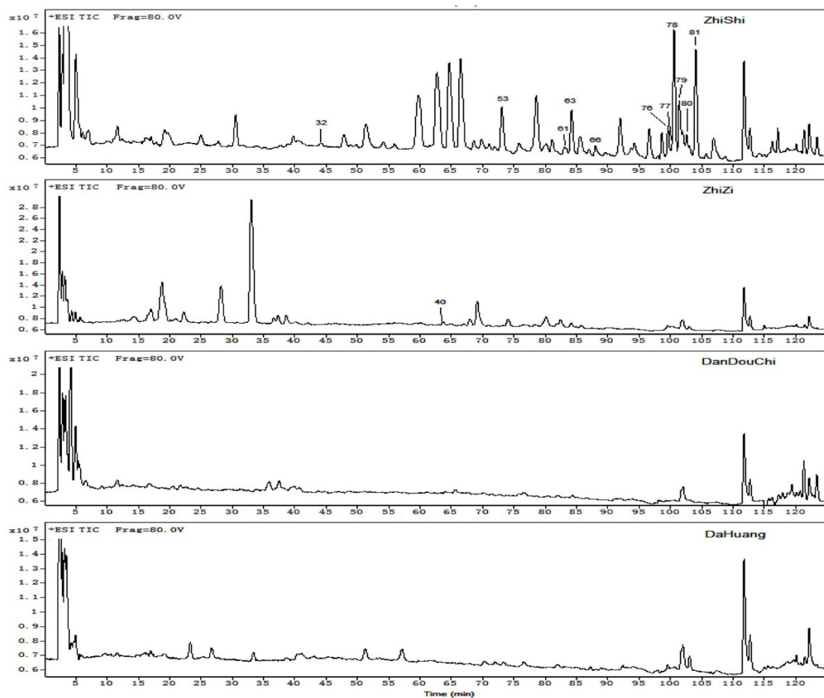
Fig. A (2) The total ion chromatograms of four individual herbs in positive ion mode.
