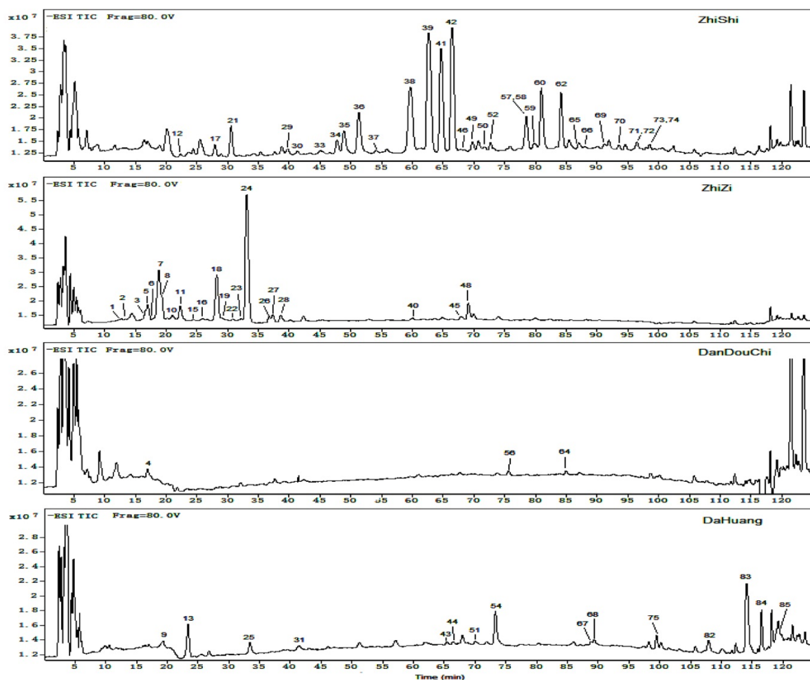
Fig. A (1) The total ion chromatograms of four individual herbs in negative ion mode.
