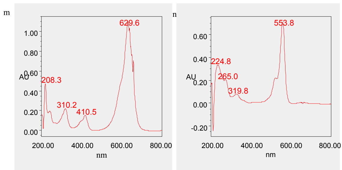
Figure S1 the UV-visible spectra of dyes: a, tartrazine; b, new red; c, amaranth; d, indigotine; e, ponceau 4R; f, sunset yellow; g, allura Red; h, carmoisine; i, acid green; j, brilliant blue; k, erythrosine; l, acidrose red B; m, patent blue V; n, rose bengale.
