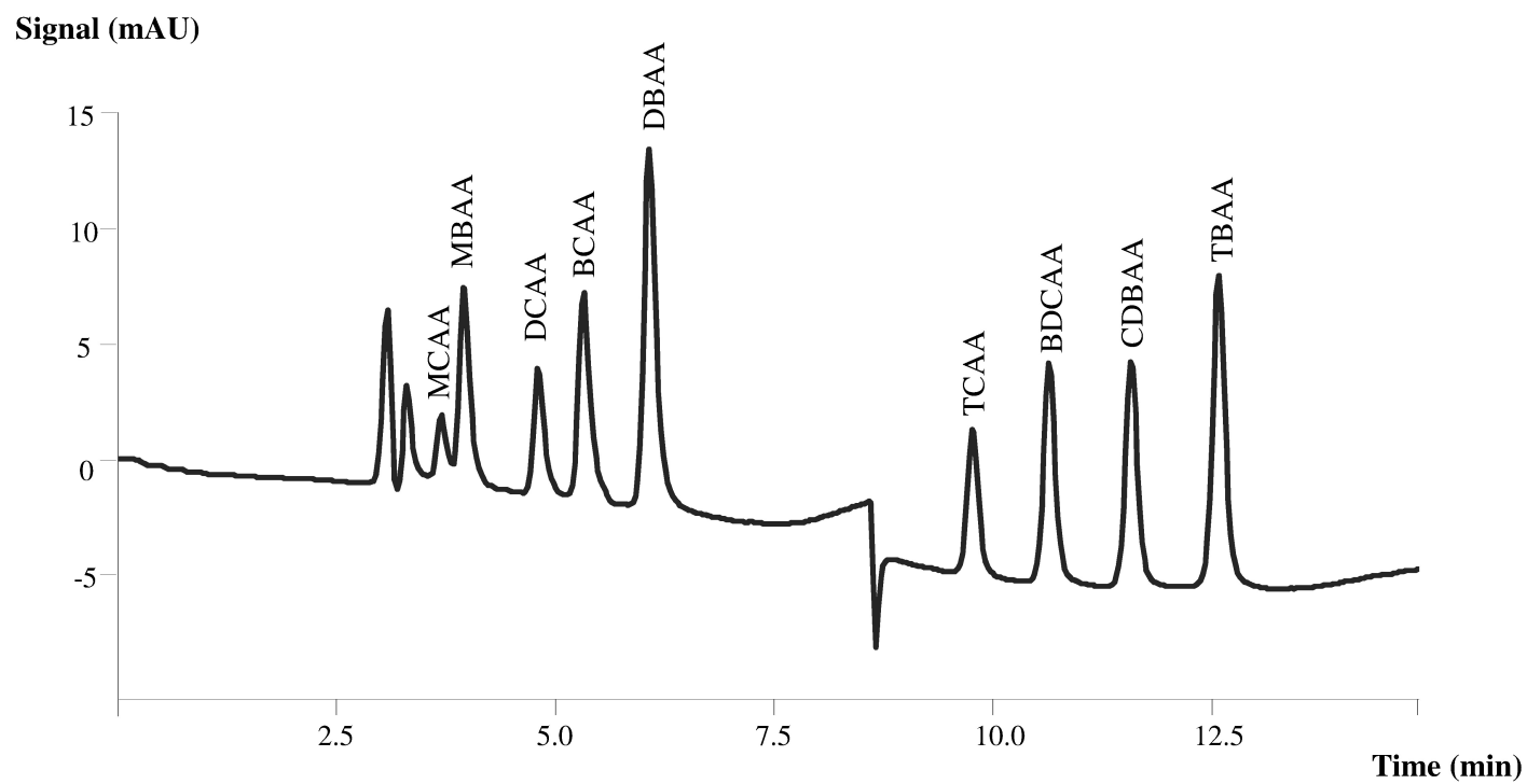
Fig. S1 Representative chromatogram of a standard mixture of HAAs (with a concentration of 10 \text{ mg}\cdot\text{L}^{-1} ) under optimum conditions.
