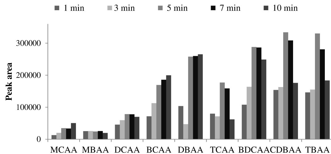
Fig. S3 Effect of the vortex in the overall VAEME method followed by the back-microextraction (1:1 ratio) when using isopropyl ether as the extractant solvent
