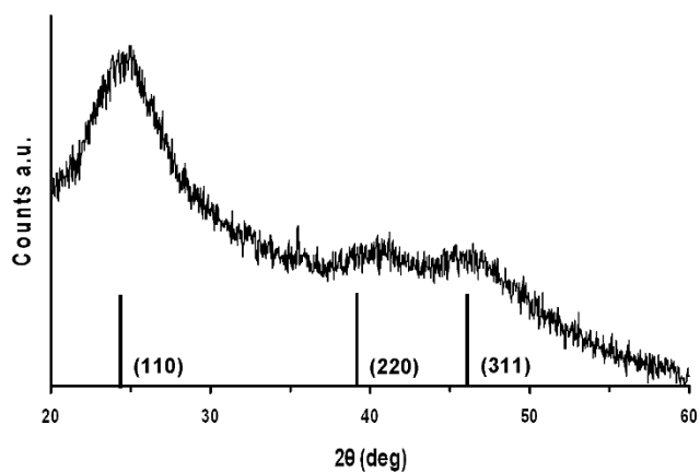
Figure S1. p-XRD of 3.1 nm CdTe-MPA QDs.
