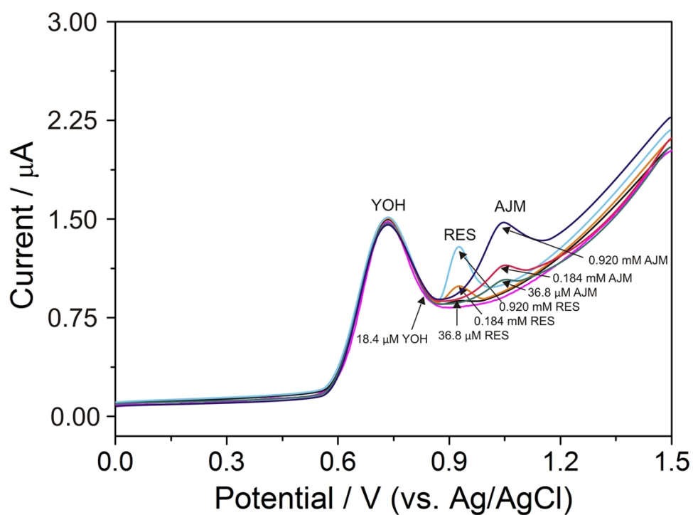
S1 Effect of the presence of reserpine (RES) and ajmalicine (AJM) in their concentration excess of 2:1 (36.8 \mu\text{M} ), 10:1 (0.184 mM) and 50:1 (0.920 mM) on current response of 18.4 \mu\text{M} YOH.
