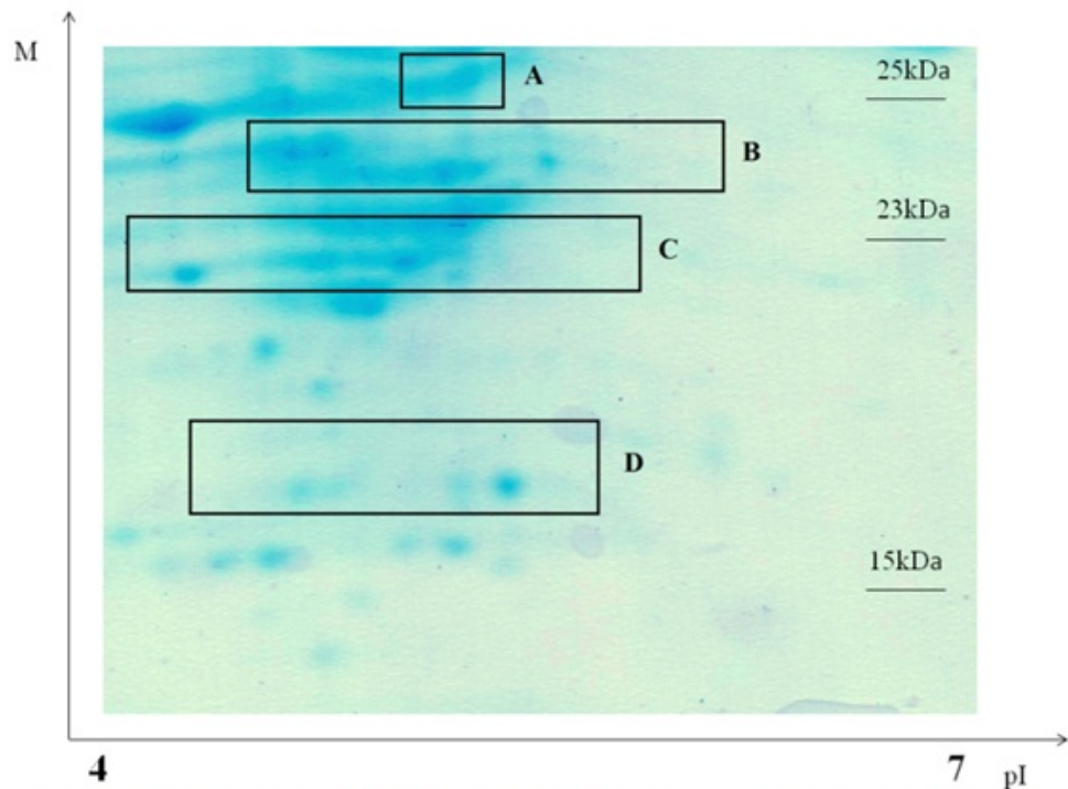
Supplement 1. 2-D gel of casein from bovine milk; the first dimension was IEF on 7 cm pH 4-7 IPG strips and the second dimension was SDS-PAGE on 12% gels (10×10 cm); the spots of proteins were stained with Bio-Safe Coomassie, excited and analyzed in spectrometric analysis. A) \alpha_{s2} -; B) \beta -; C) \alpha_{s1} - and D) \kappa -casein
