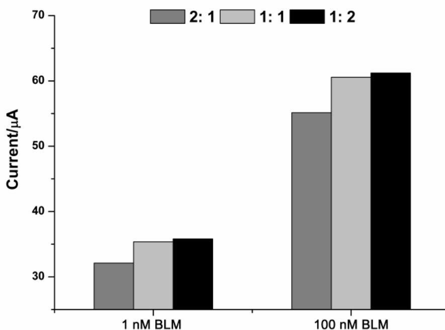
Fig. S1 Effect of molar ratio of BLM and Fe 2+ on DPV peak currents.
