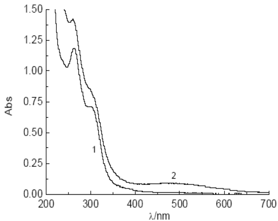
Figure S2 UV-Vis spectra of PA (Fig.S2) in the (1)absence and (2)presence of \text{Fe}^{3+} .
