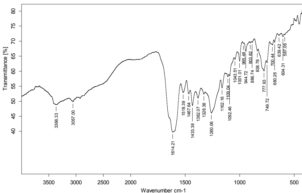
Figure S1: FT-IR of chemical PA
