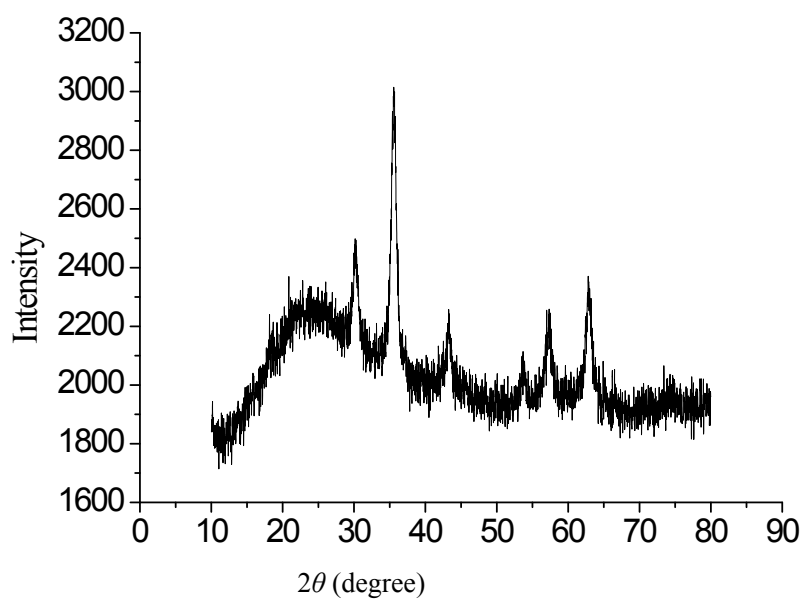
Figure S1. X-ray diffraction pattern of the MOPC-ZSM-5.
