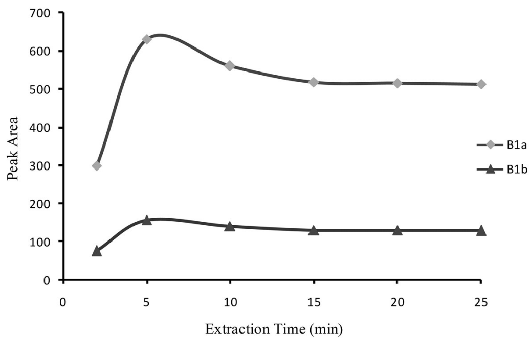
MSPE time profiles of avermectines B 1a and B 1b using PPy/MNP sorbent
