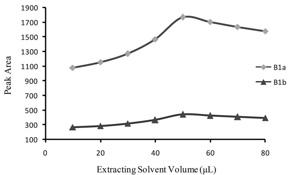
Effect of extracting solvent volume on the DLLME efficiency
