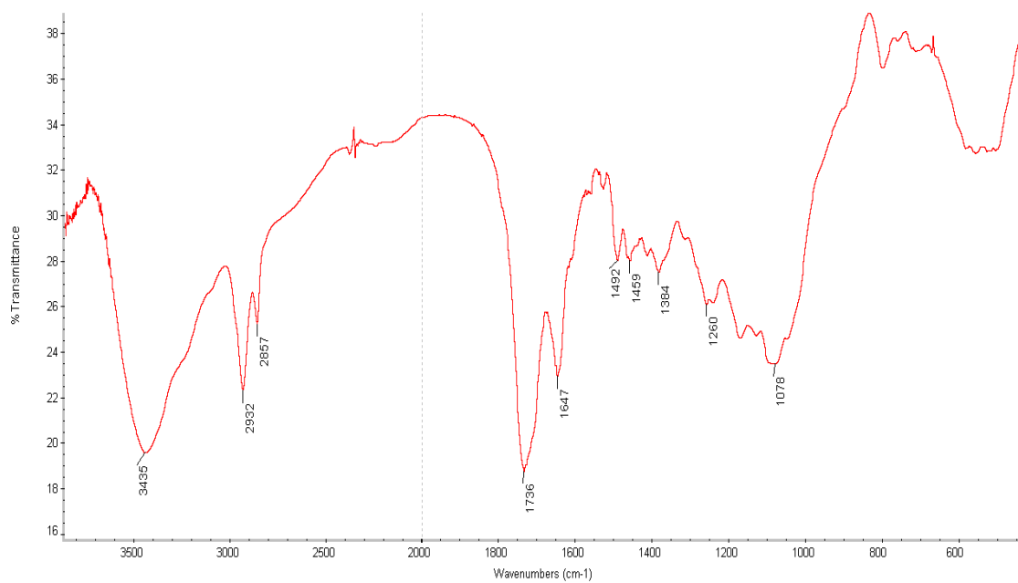
Fig. S1 FTIR spectrum for poly (VAF-co-VSC-co-VGA)
