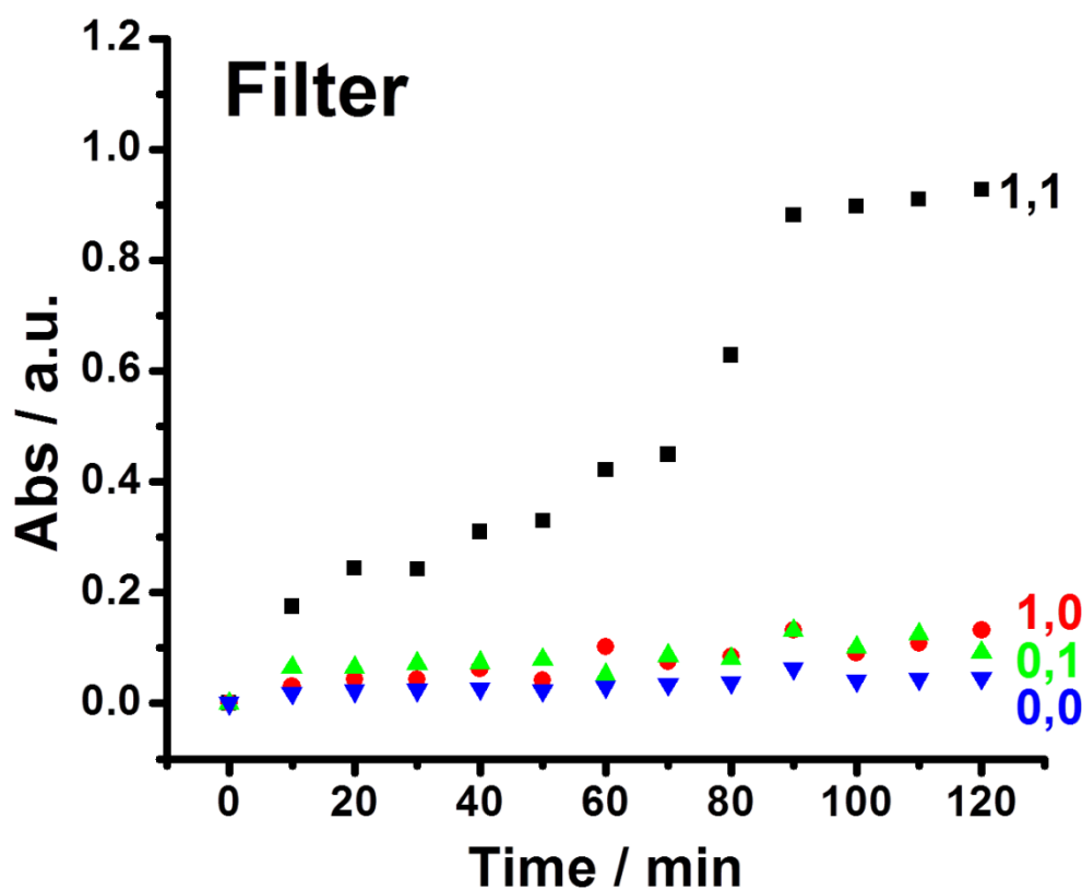
Figure S1. The kinetics of the production of citric acid from the biocatalytic cascade for all input combinations in the presence of the filter
