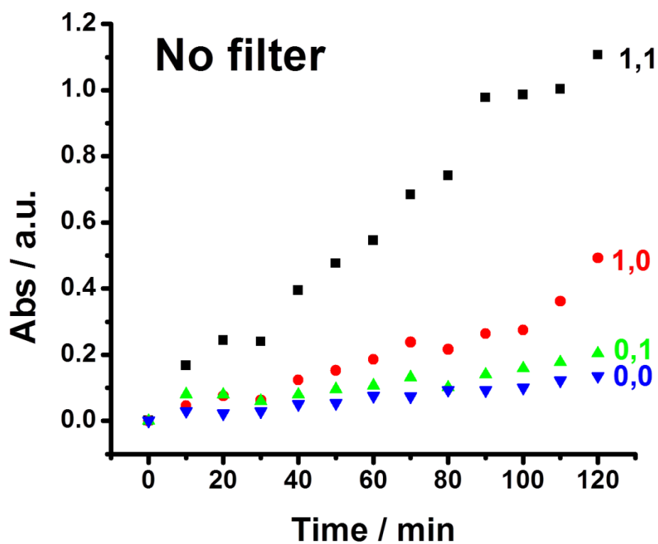
Figure S2. The kinetics of the production of citric acid from the biocatalytic cascade for all input combinations in the absence of the filter
