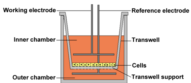
Figure S1. The cell-device system in impedance measurement.
