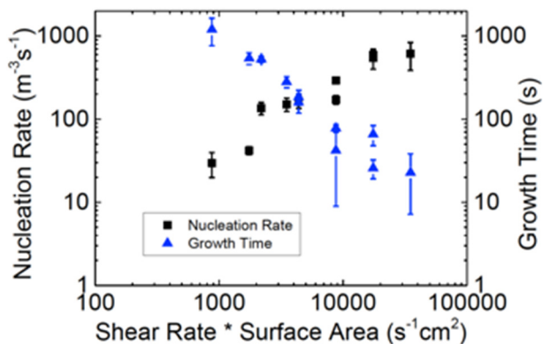
Figure 1.1 Induction time (s), nucleation rates J , and growth times t_g estimated from a model fit as a function of the product of the average shear rate and surface area. Adapted from ref. 34 with permission from American Chemical Society, Copyright 2015, and ref. 35, https://pubs.acs.org/doi/abs/10.1021/acs.cgd.5b01042 , with permission from American Chemical Society, Copyright 2016.
