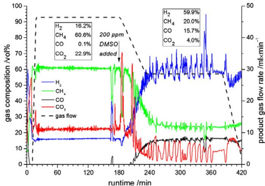
Figure 7.7 . Flow rate and composition of product gas during the gasification of 7.5% ethanol in SCW (400 °C and 24.5 MPa). DMSO was added after 180 min and DI water was fed from 370 min onward. Reproduced from Ref. 50 with permission from Elsevier, Copyright 2004.
