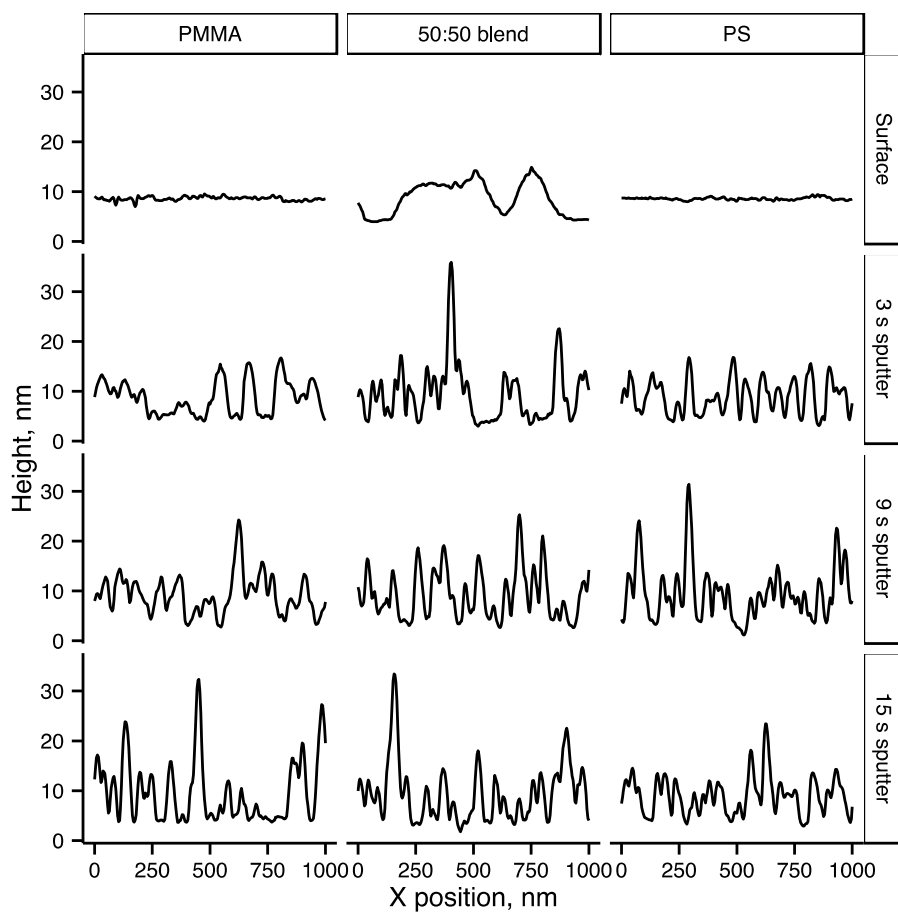
Supplementary figure 1: Horizontal line scans across the center of representative AFM images of sputter craters in polymer films presented in figure 5.
