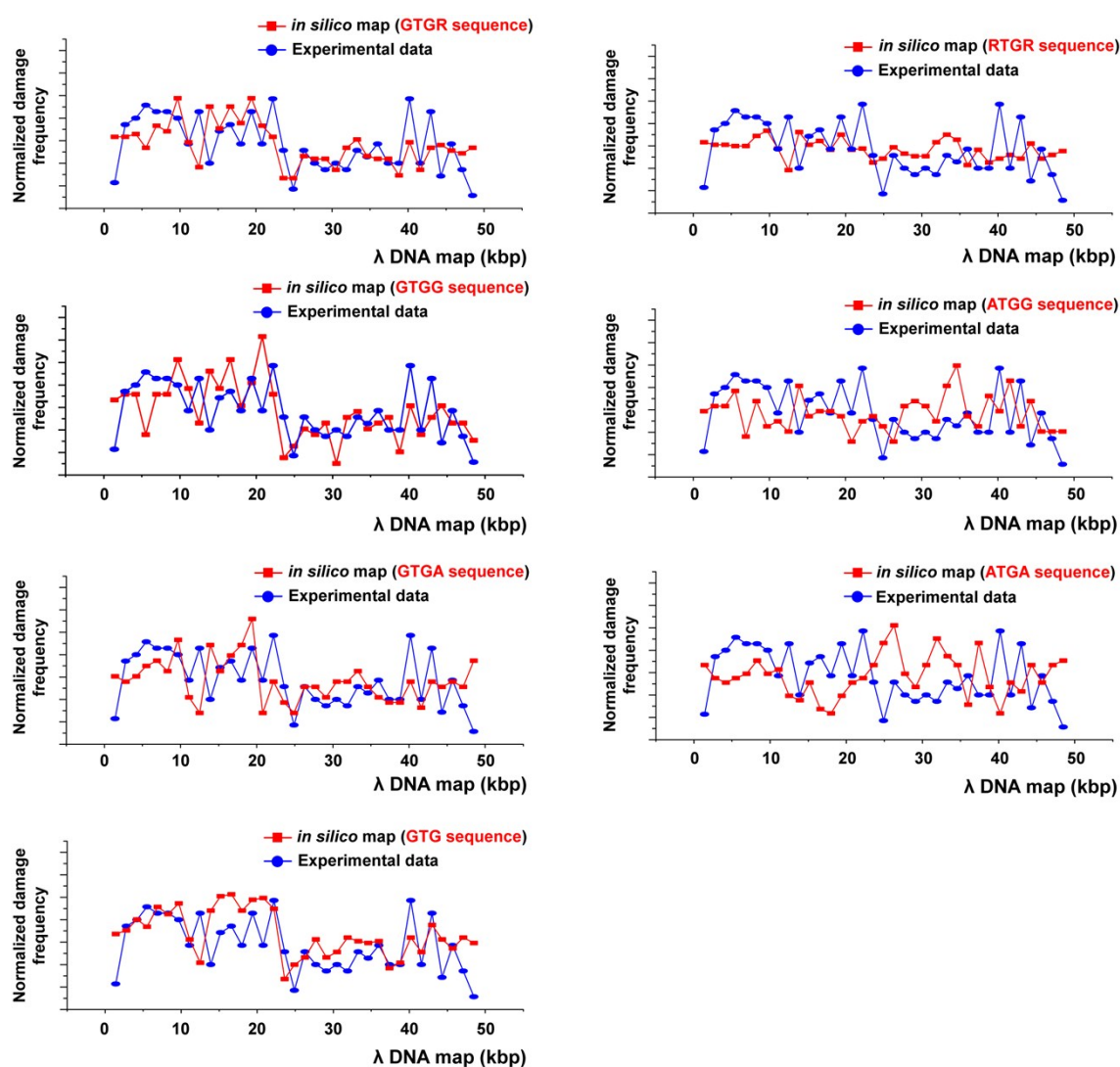
Figure 1 Comparison of in silico sequence frequency map (■) and damage frequency map (●)
