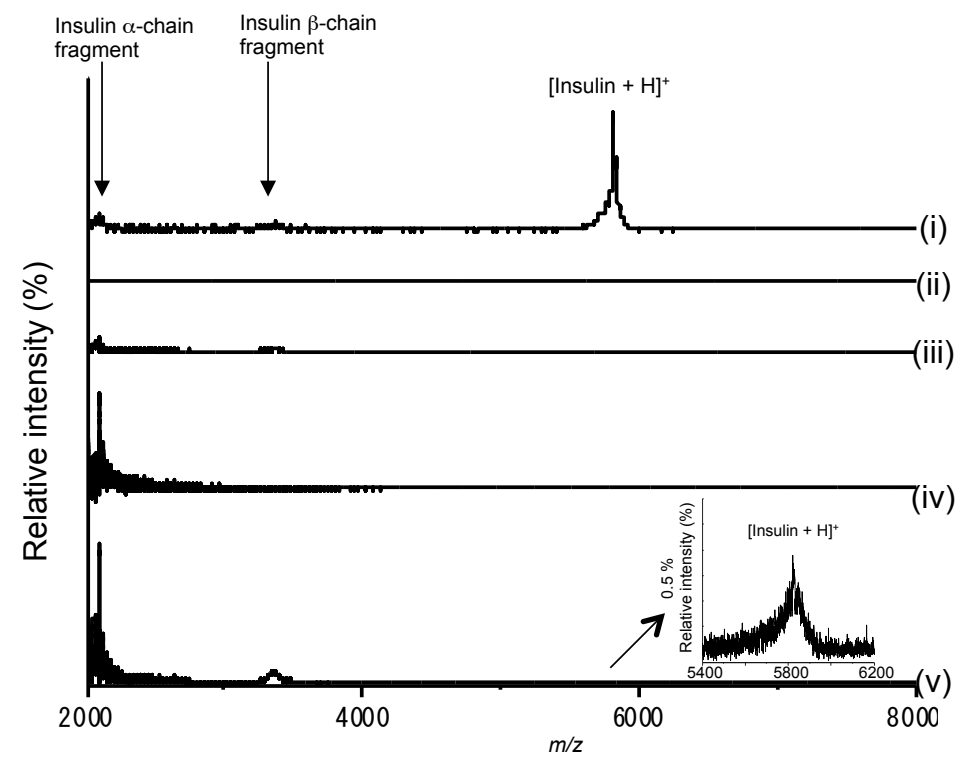
S2 MS spectra of insulin that was ionized by SA-NP (i) DHB-NP (ii) and CHCA-NP (iii) at 11 [J] and, DHB-NP (iv) and CHCA-NP (v) at 60 [J] .
