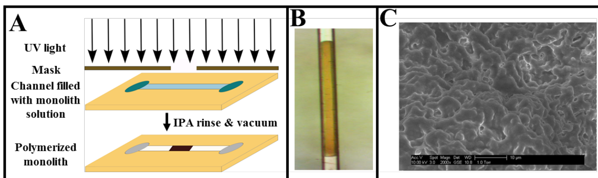
Figure S1. C8 monolith fabrication. (A) Schematic showing fabrication. (B) Photograph of a C8 monolith in a COC channel. (C) SEM image showing internal structure of a C8 monolith.
