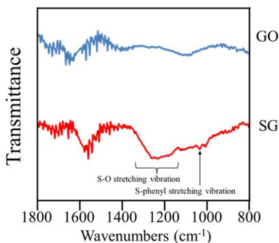
Fig. S2 FT-IR spectra of GO and SG. (FT-IR spectra were obtained by using JASCO FT/IR-4200.)
