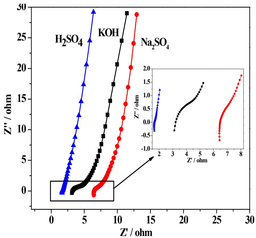
Fig. S3 EIS plots of TiN NTA electrode in 1mol/L H 2 SO 4 , KOH and Na 2 SO 4
