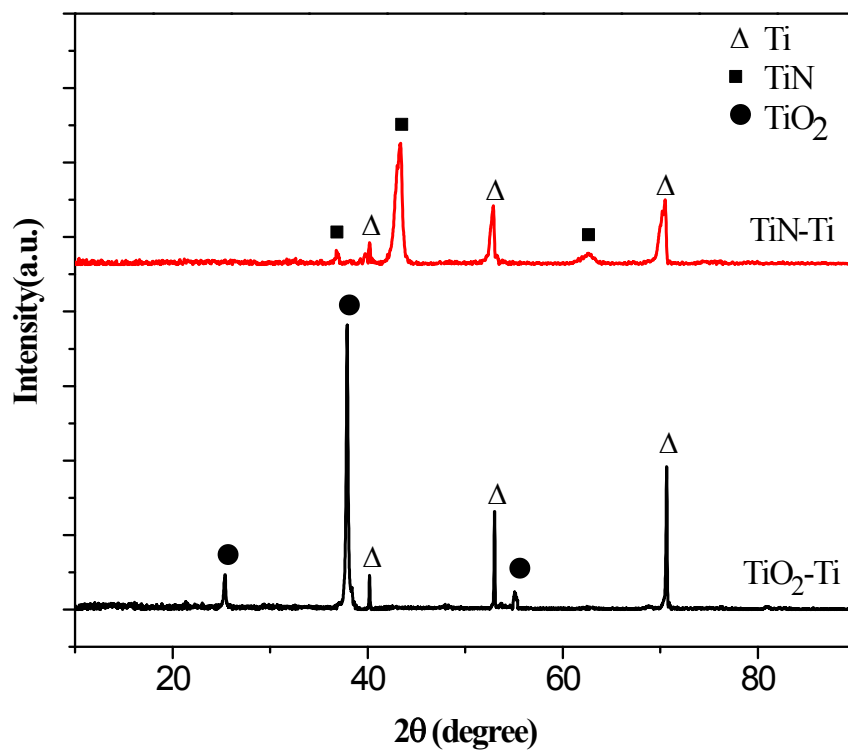
Fig. S1 XRD patterns of \text{TiO}_2 NTA and TiN NTA on the Ti sheet
