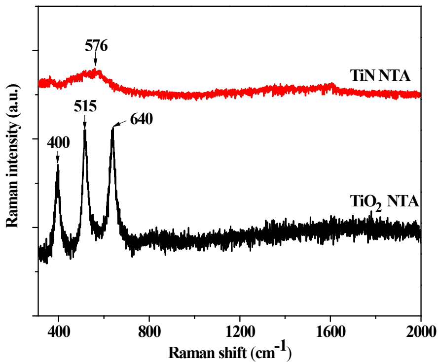
Fig. S2 Raman spectra of \text{TiO}_2 NTA and TiN NTA
