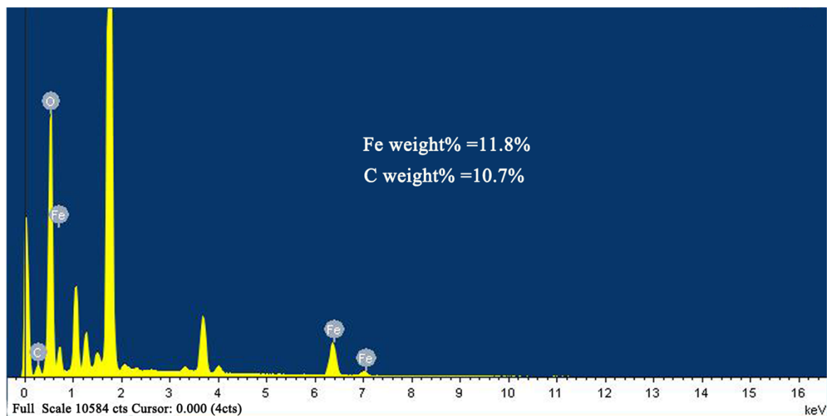
Figure S2 Contents of iron and carbon elements in β-CDEP-modified Fe 3 O 4 microspheres by EDX spectroscopy analysis.
