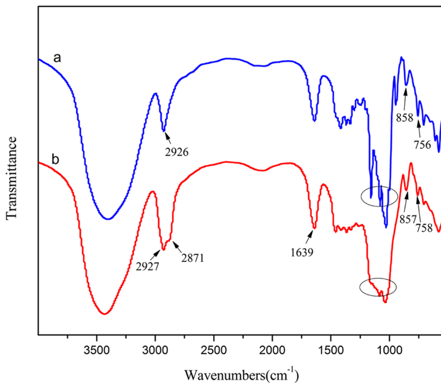
Figure S1 FT-IR spectra of (a) β-CD and (b) β-CDEP.
