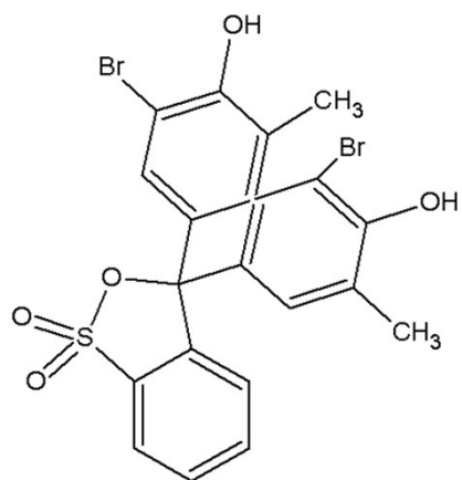
Fig. S1 The structure of bromocresol purple (5,5'-Dibromo-o-cresolsulfonphthalein)
