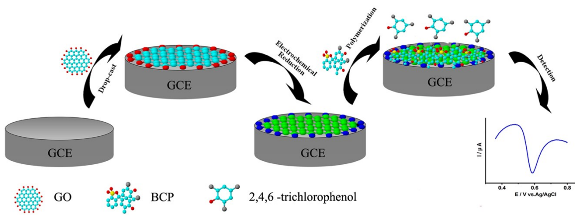
Fig. S2 Schematic diagram of the fabrication procedure of BCP/erGO/GCE
