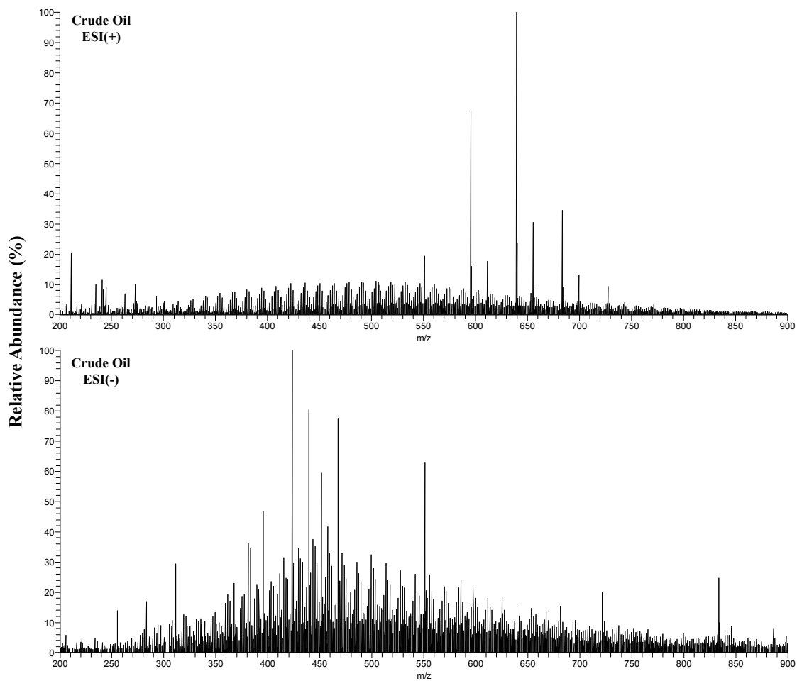
Figure S1. Total mass spectrum by ESI( \pm ) FT-ICR MS for crude oil. A high intensity of contaminant ion peaks seriously hampered data analysis, preventing the proper classification of species.
