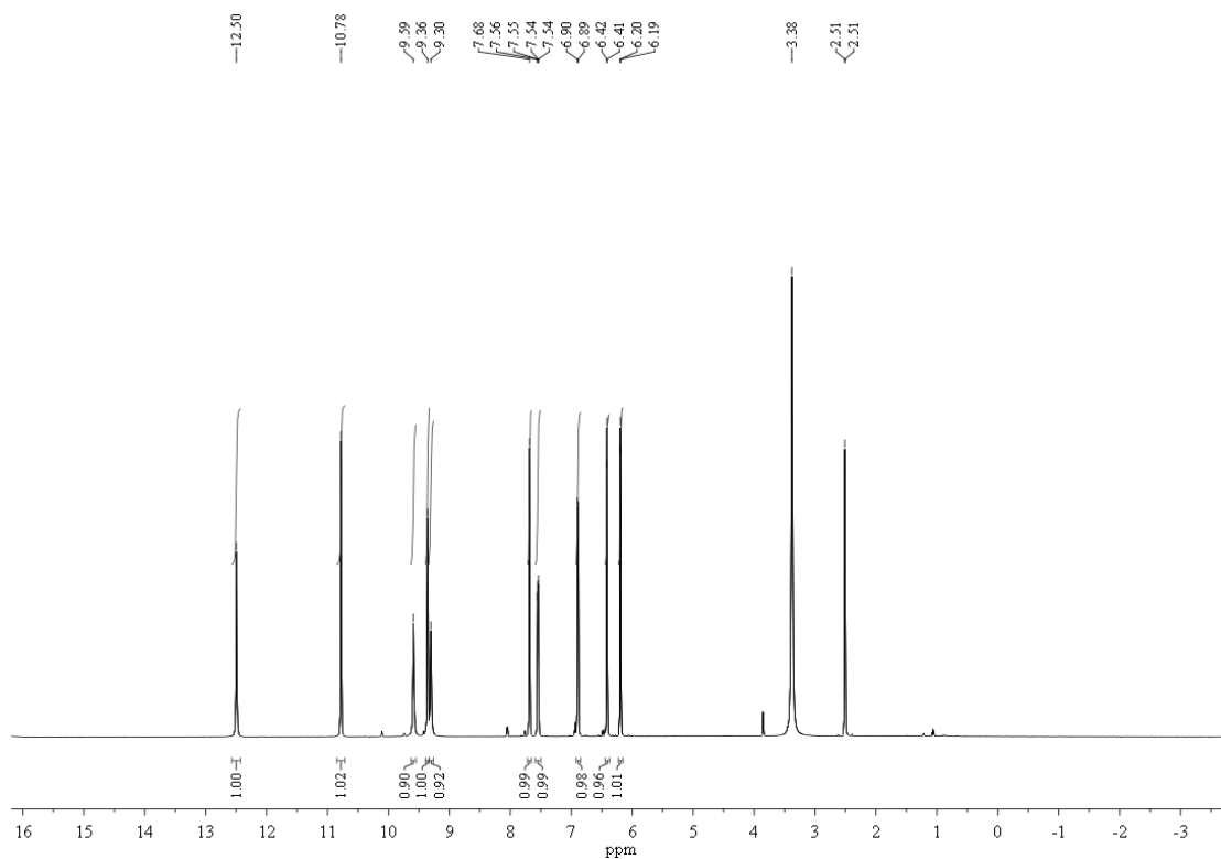
Fig.S2 The ^1\text{H} NMR of Q
