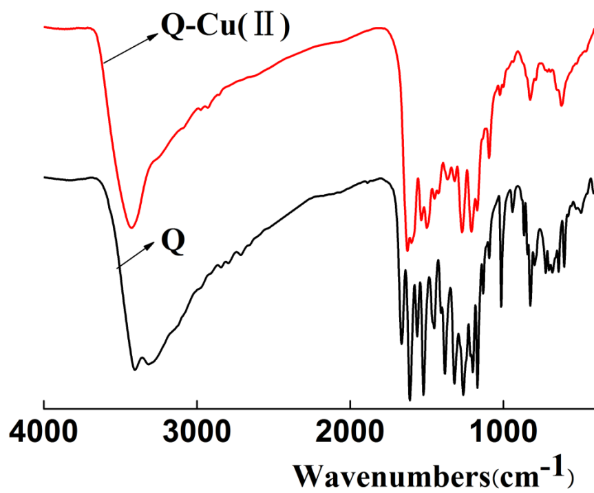
Fig.S3 The FTIR spectrum of Q and Q-Cu(II)
