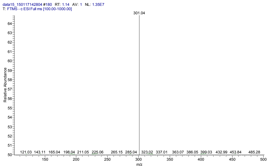
Fig.S1 The mass sepcturm of Q
