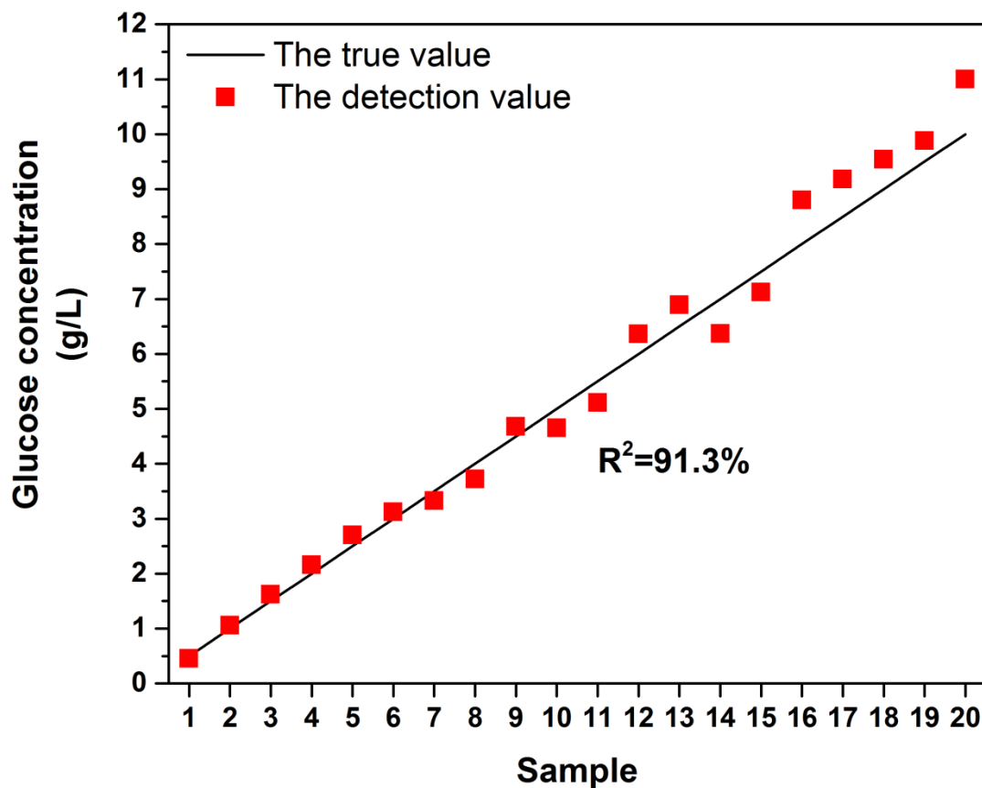
Figure S1: The accuracy validation experiments for nonlinear fitting algorithm for glucose detection. The detection results and the true concentrations of 20 samples were used for comparison.
