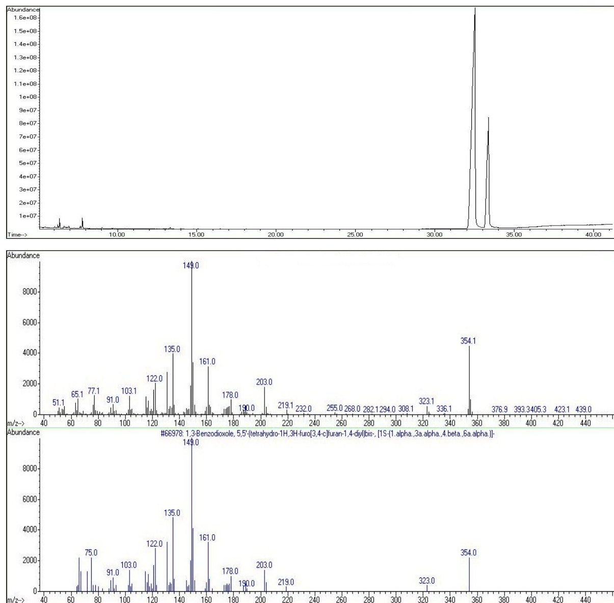
Figure S1. (Top) Full scan chromatogram of sesame oil after clean-up with EZ-POP NP; (Bottom) mass spectrum of major interfering compound (retention time = 32.52 min) and reference spectrum from NIST library.
