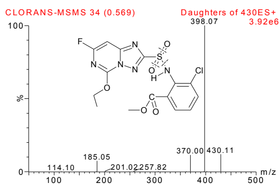
Fig.1. the structures showing the fragmentation for the representative analytes in MS/MS mode
