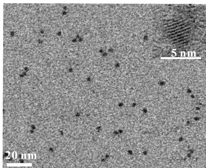
Figure S1. TEM image of QDs (inset: the HRTEM image).
