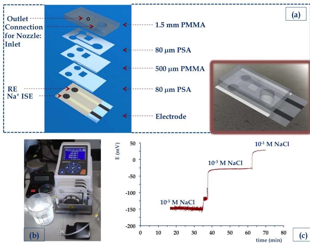
Figure SID. 1: (a) 1 st generation of the Microfluidic unit integrated on top of the screen-printed electrodes and (b) the experimental set-up used to carry out the first on-bench tests (i.e. potentiometric strip connected to a peristaltic pump). (c) Example of a three-point calibration curve realised using the set-up in (b).
