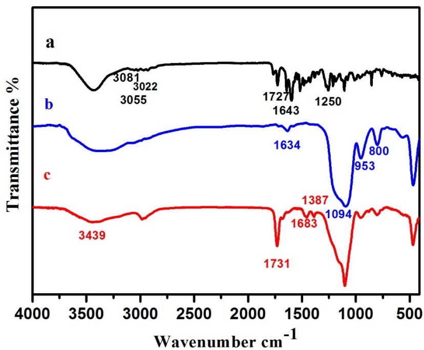
Fig. S2 FT-IR spectra of (a) allyl fluorescein, (b) SiO 2 -MPS, (c) SiO 2 -MPS@FMIP
