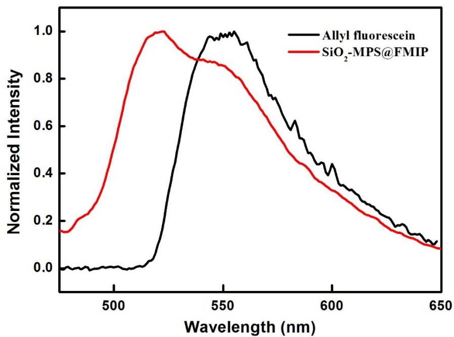
Fig.S4 Fluorescence spectra of allyl fluorescein and SiO 2 -MPS@FMIP
