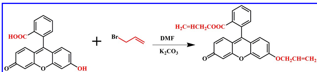
Fig S1 Synthetic scheme for allyl fluorescein
