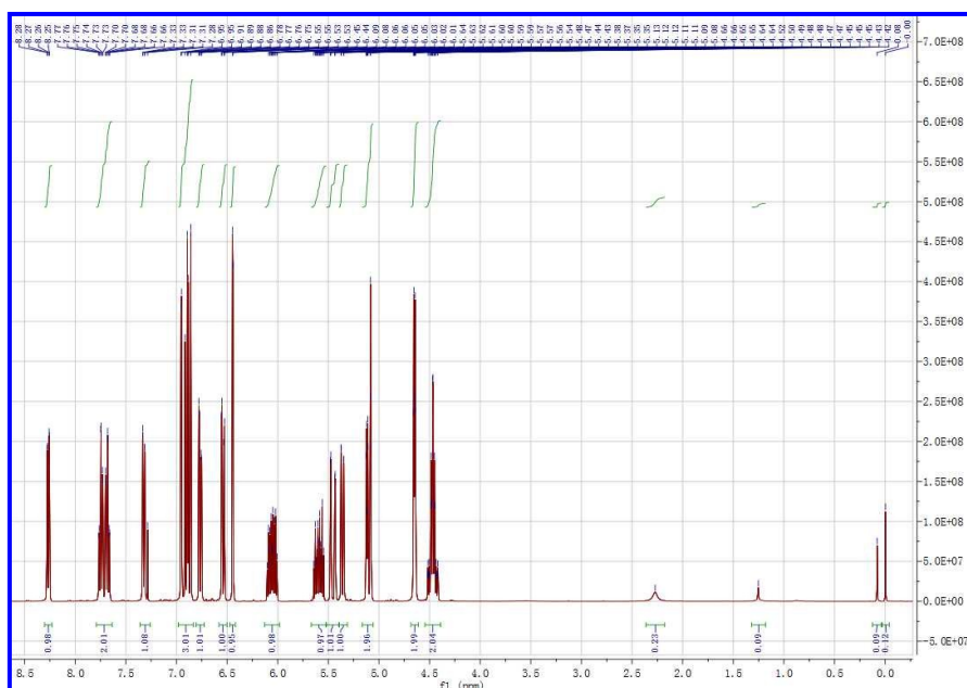
Fig S3 1 H-NMR spectroscopy of allyl fluorescein
