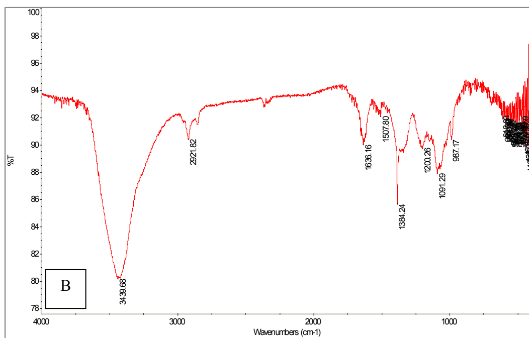
The FT-IR spectra of GO (A) and ERGO (B).
