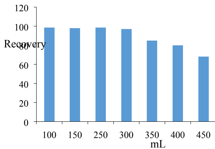
Fig. 1 S Effect of sample volume on extraction recovery
