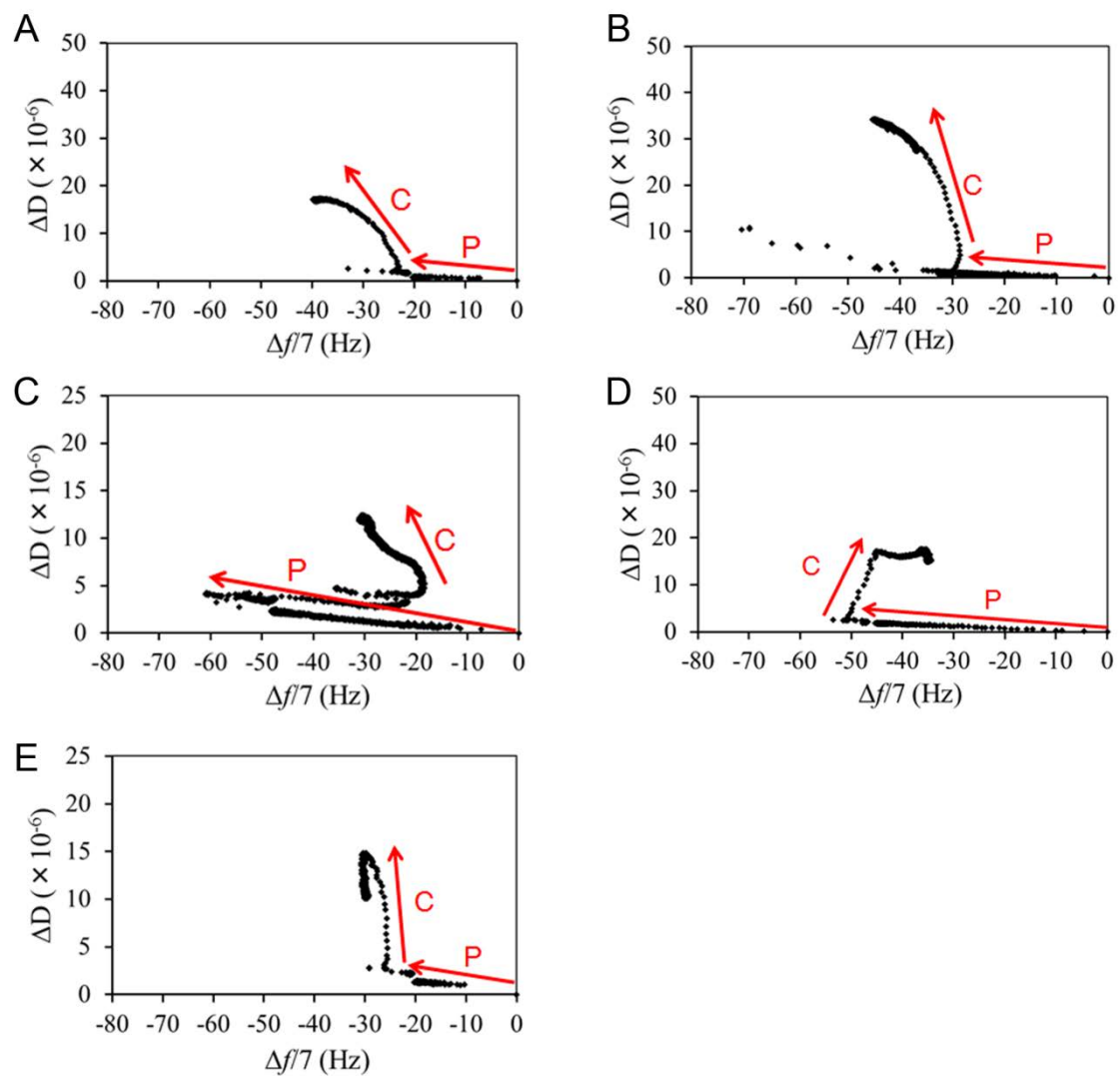
Fig. S2. Alternative QCM-D \Delta D - \Delta f plots for (A) the CH 3 -SAM surface, (B) the NH 2 -SAM surface, (C) the SiO 2 surface, (D) the COOH-SAM surface and (E) the OH-SAM surface. "P" denotes the protein adsorption phase, and "C" denotes the cell adhesion phase.
